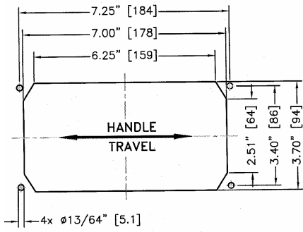
2020 "CUT-OUT" DIMENSIONS 1 ENGINE
